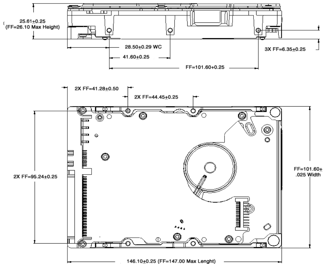
Figure 3-6 Mounting Dimensions Maxtor Atlas 15K II Drives
