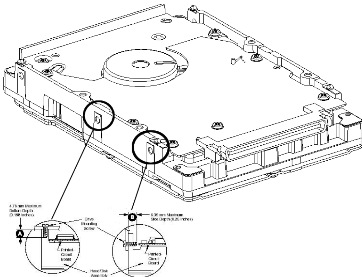
Figure 3-7 Mounting Screw Clearance for Maxtor Atlas 15K II Drive
